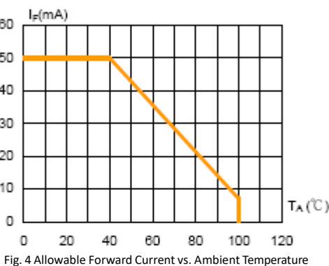
Fig. 4 Allowable Forward Current vs. Ambient Temperature
