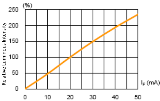
Fig. 2 Luminous Intensity vs. Forward Current
