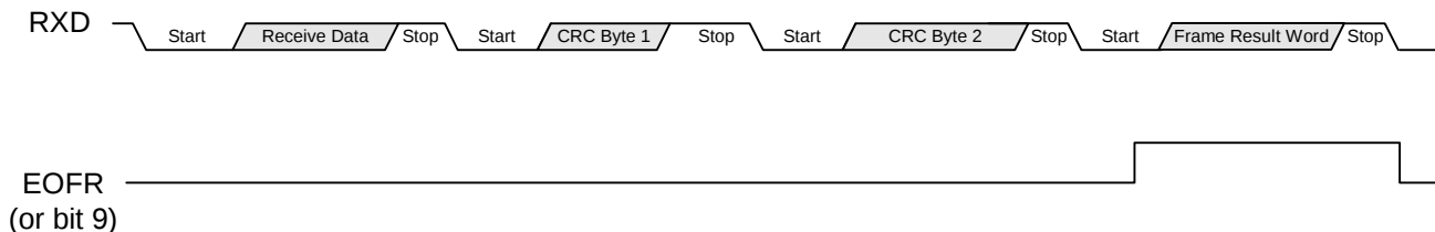
B. Frame Receive
