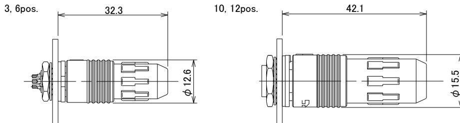
Mating Diagram
