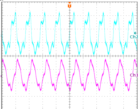
Output voltage ripple at nominal input voltage and max load current Top trace +15V, 10 mV/div, Bottom trace -15V, 20mV/div, 2us/div.
