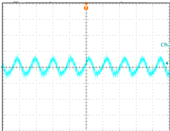
Output voltage ripple at nominal input voltage and max load current (4mV/div, 2us/div) Load cap: 10μF, tantalum capacitor and 1μF ceramic capacitor. Bandwidth: 20 MHz.
