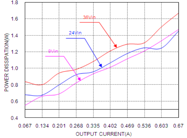
Power dissipation vs. load current at 25°C.
