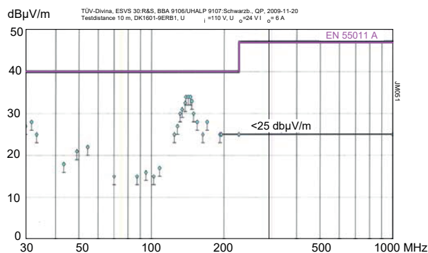
Fig. 23b Typical radiated emissions according to EN 55011/32, antenna 10 m distance, measured at V_{inom} and I_{o nom} (DK1601-9ERB1)
