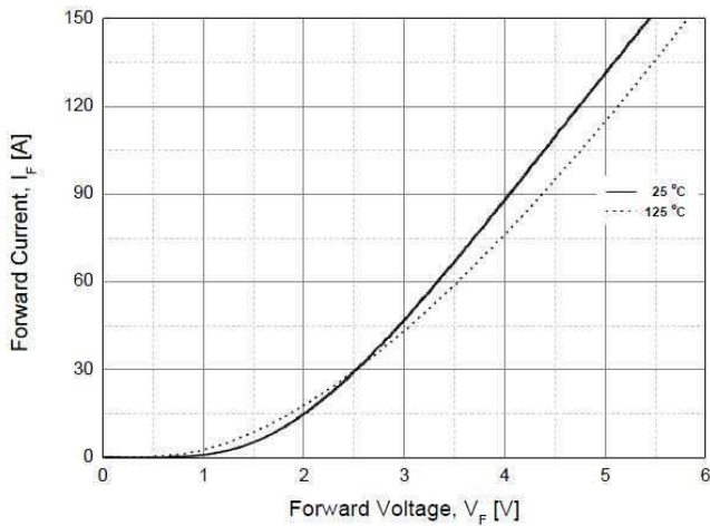
Conduction Characteristics
