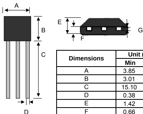
TO-92S
