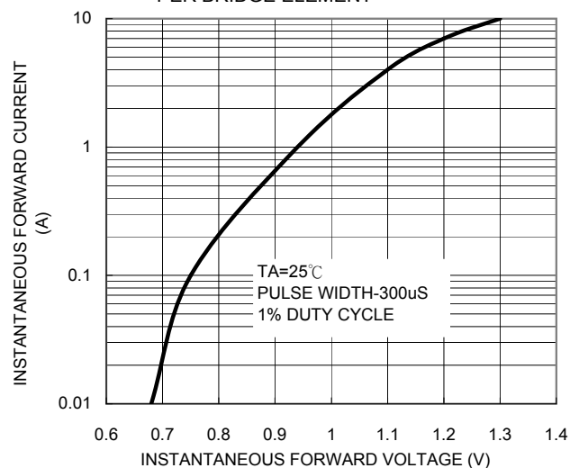
FIG. 5- TYPICAL FORWARD CHARACTERISRICS PER BRIDGE ELEMENT
