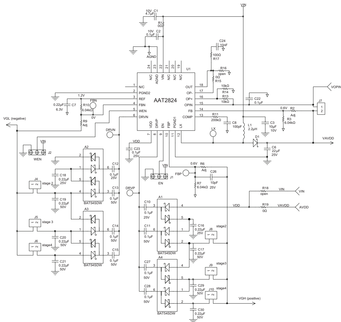
Figure 8: AAT2824IBK Evaluation Board Schematic.
