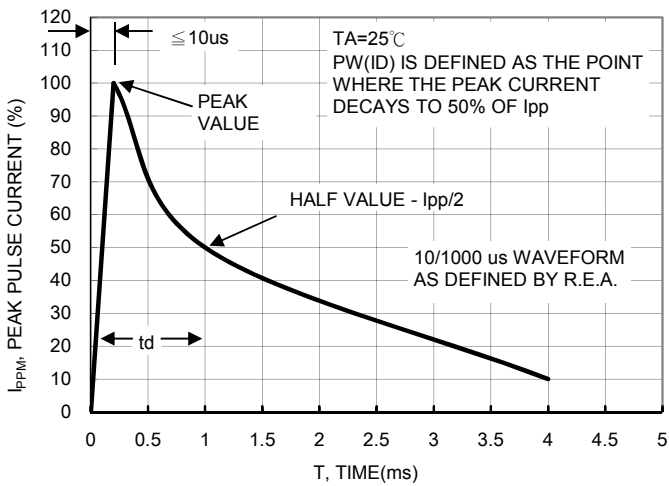
FIG. 7 PULSE WAVEFORM
