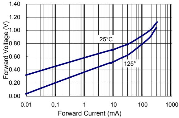
FIG 1 Forward Voltage vs Forward Current
