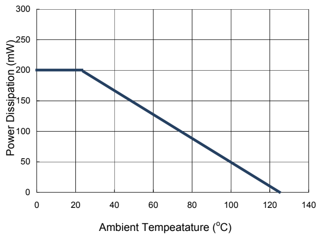
FIG 2 Admissible Power Dissipation Curve
