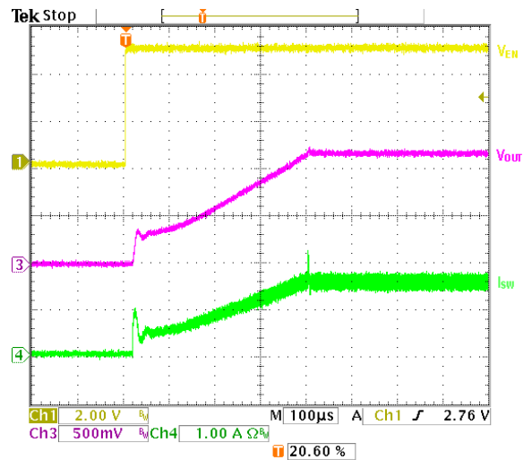
Figure 14. V_{in} = 5V , V_{out} = 1.2V , I_{out}=0\sim 2A
