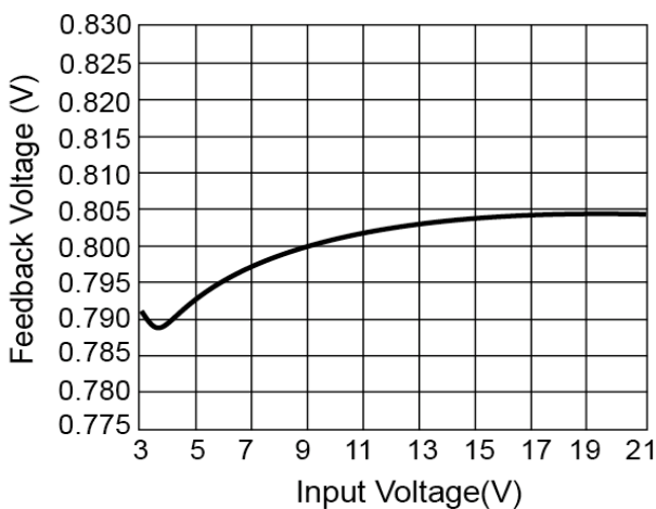
Figure 1. Feedback Voltage vs. Input Voltage
