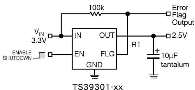
2.5V/3A Regulator with Error Flag
