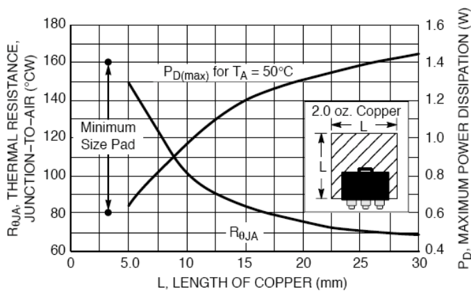
Figure 3 – SOT-223 Thermal Resistance and Maximum Power Dissipation vs. P.C.B Copper Length
