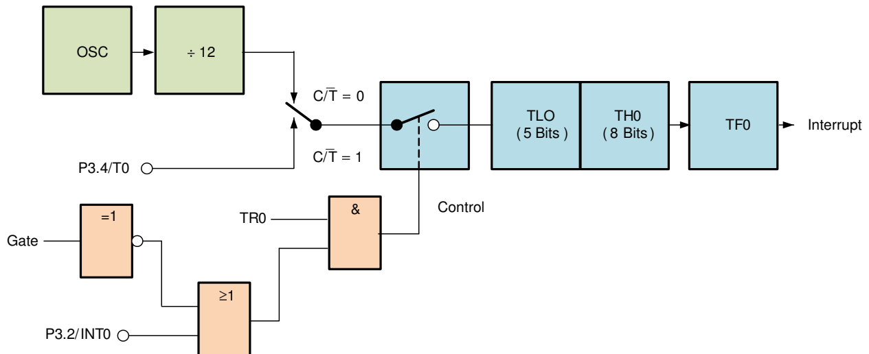
Figure 7. Timer 0 Mode 0
