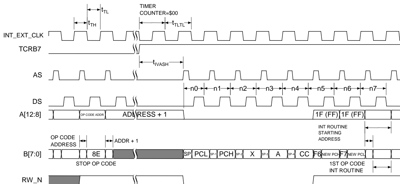
Figure 18. Interrupt Recovery From STOP Instruction Timing
