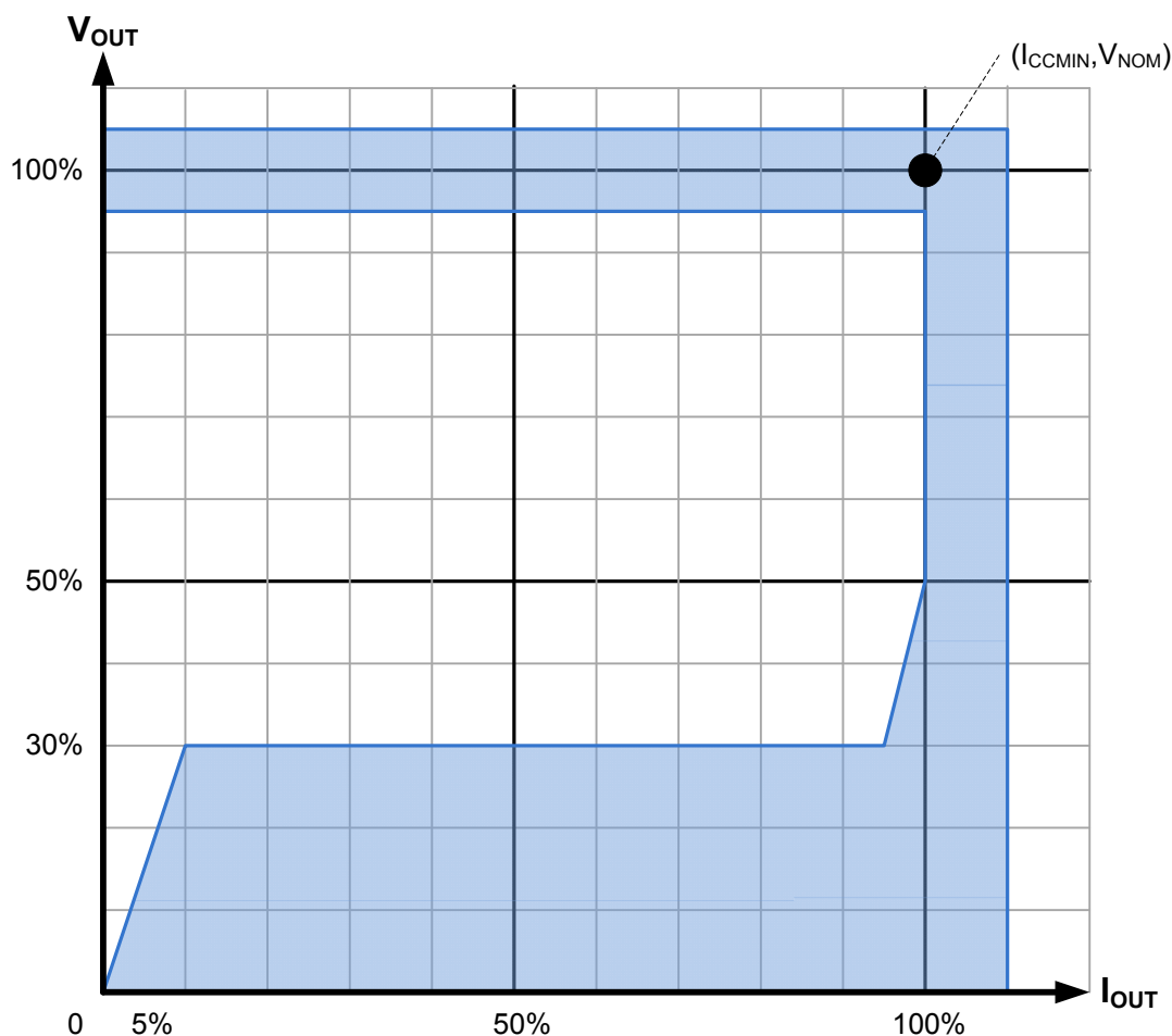
Figure 6: Achievable Charger Output Characteristic Using C2161DX2 and C2162DX2
