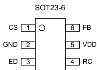
Figure 3: C2161DX2 and C2162DX2 Pin Assignment
