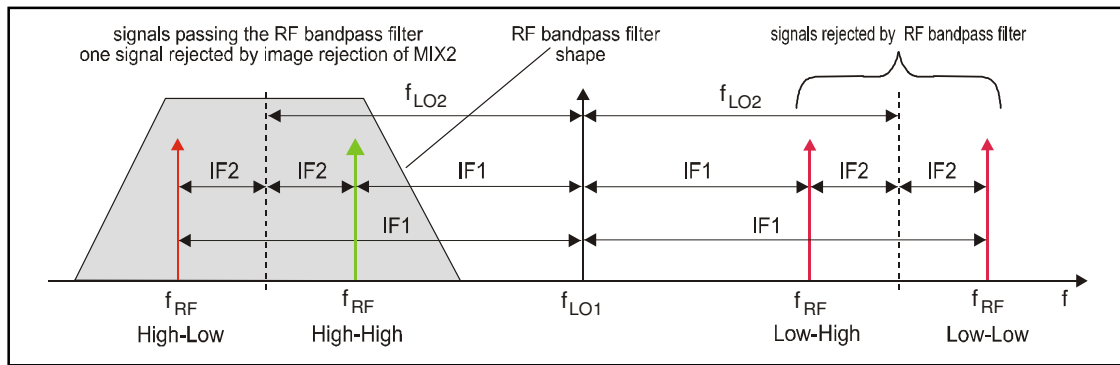
Fig. 3: The four receiving frequencies in a double conversion superhetro receiver
