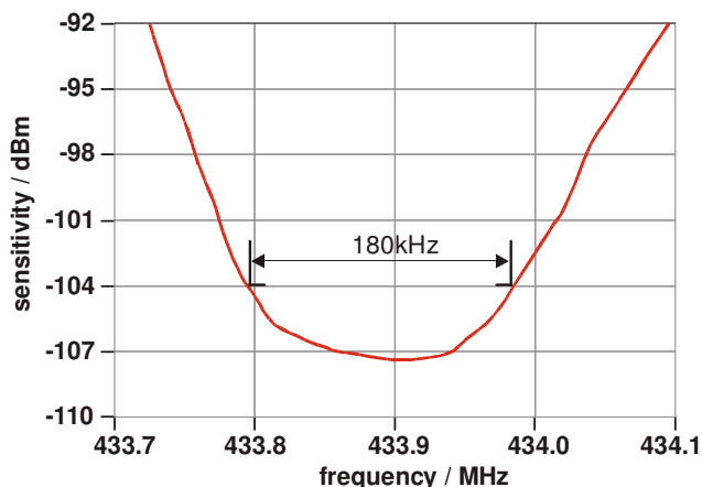
Fig. 16: Measured sensitivity characteristic (BER= 3 \cdot 10^{-3} , 4kbps, \Delta f = \pm 20kHz )
