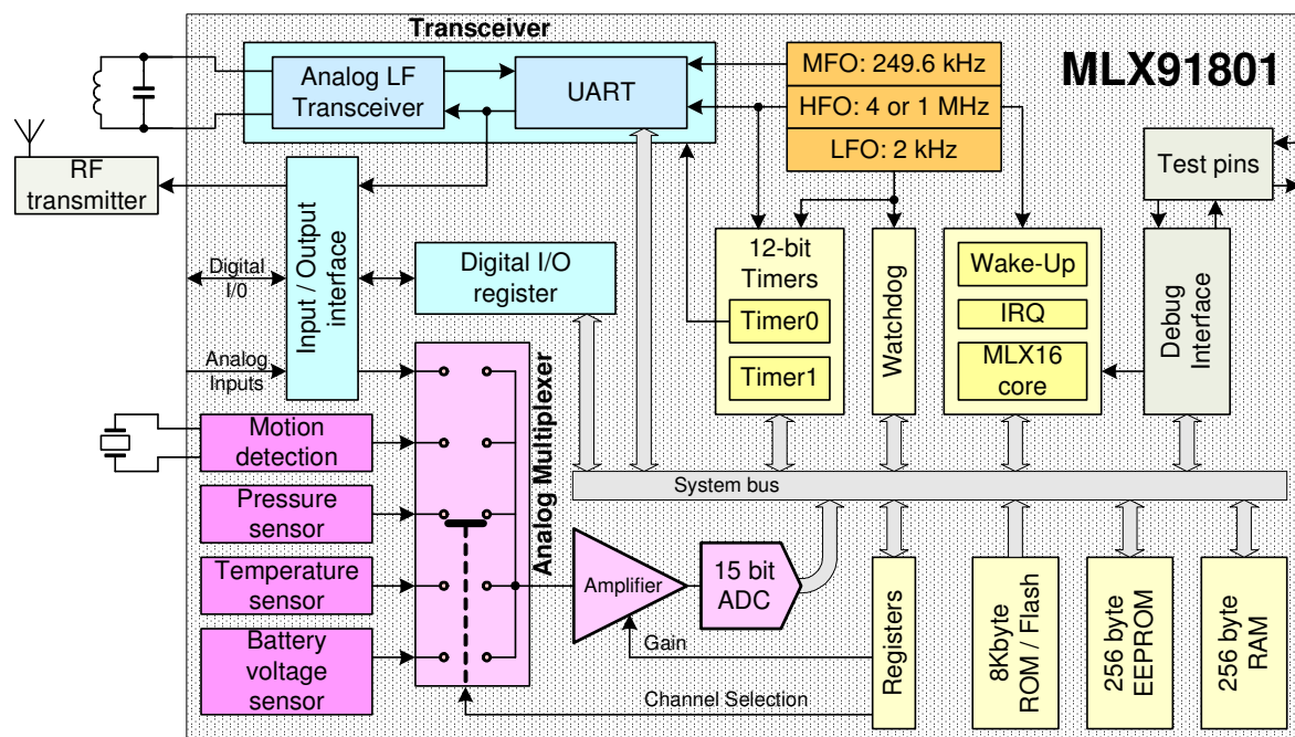
Fig. 2 MLX91801 block diagram
