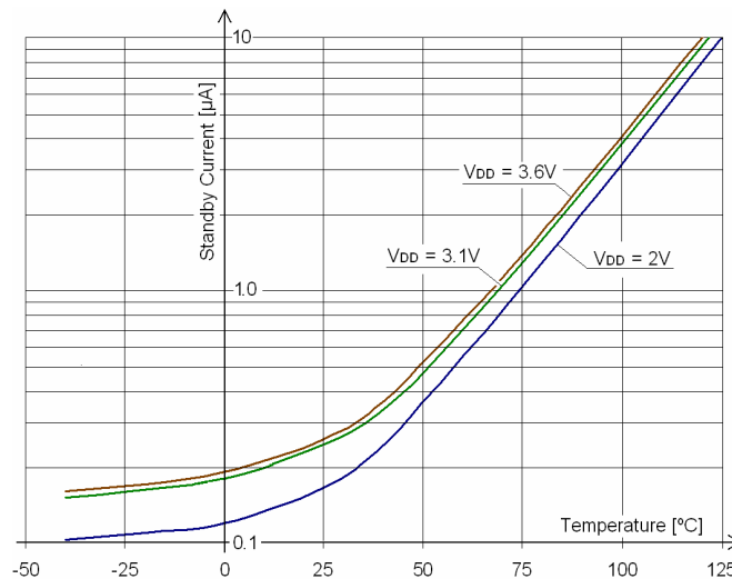
Fig. 1 MLX91801 typical standby current (internal voltage regulator is off)
