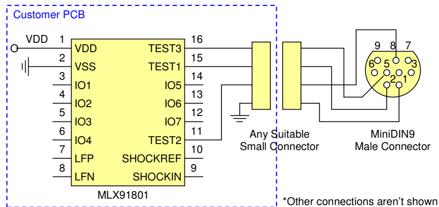
Fig. 7 Example of a MLX91801 interface with the Mini E-mlx programmer
