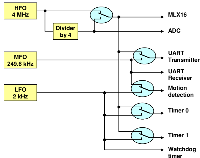
Fig. 3 MLX91801 oscillators
