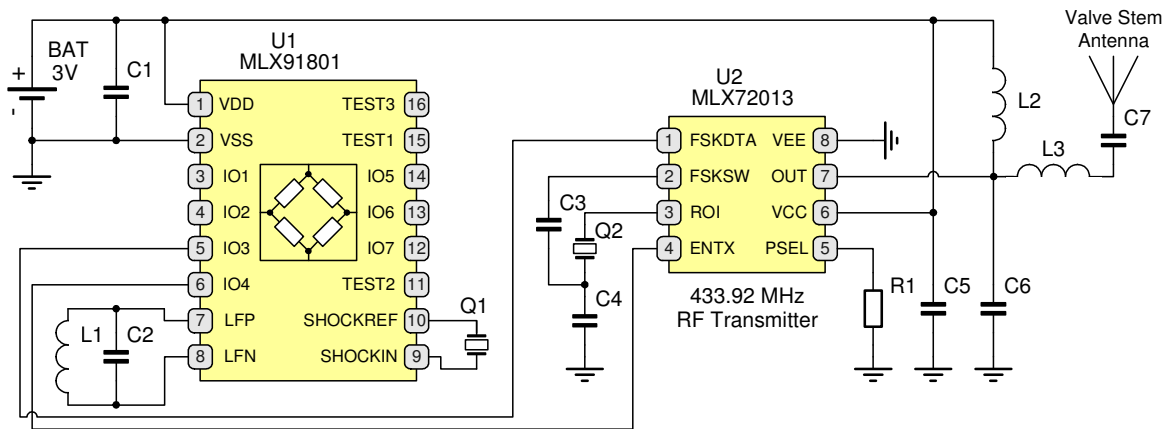
Fig. 6 Schematic example of the tire pressure sensor based on the MLX91801
