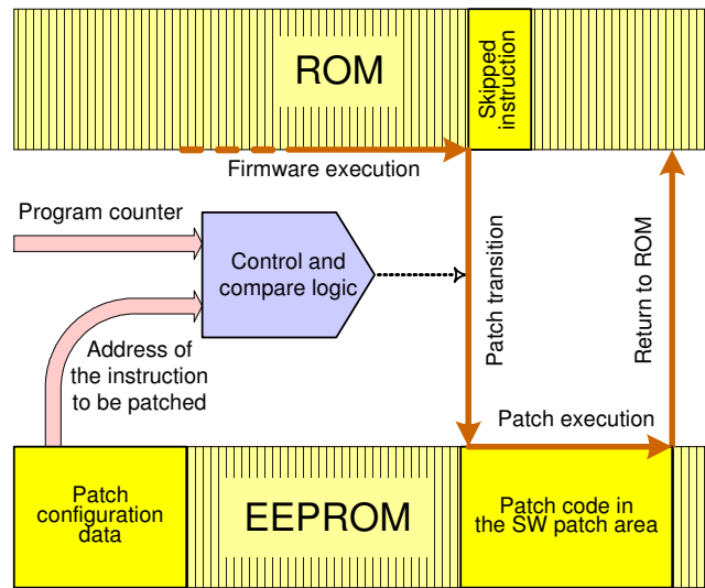
Fig. 4 Simplified patching scheme
