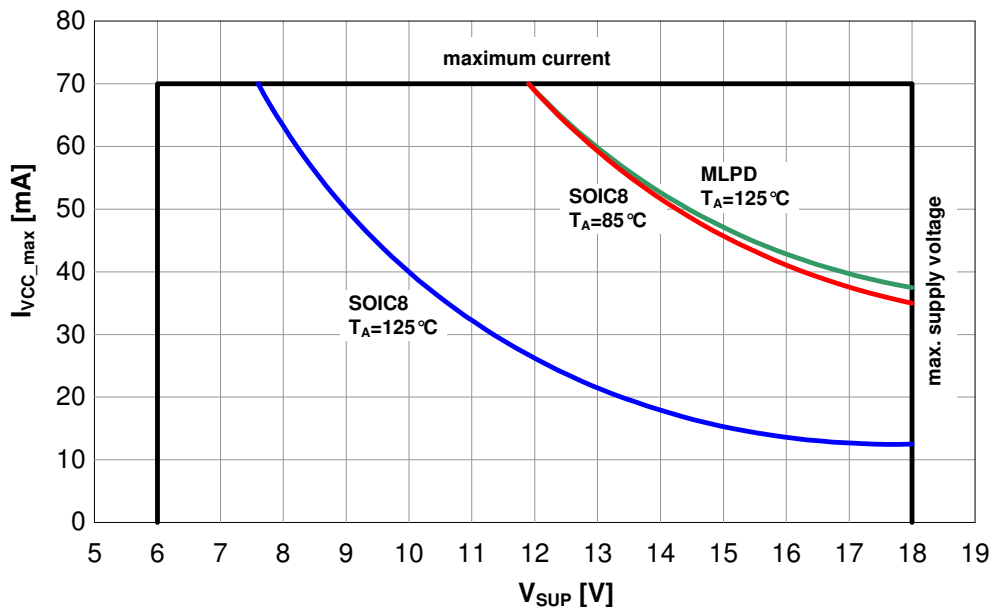
Figure 17 - Safe operating area
