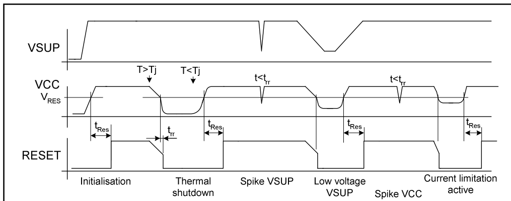
Figure 11 - Reset behaviour
