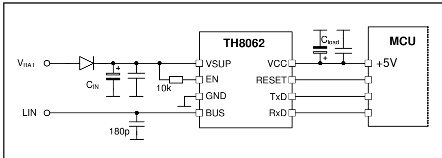
Figure 15 - Permanent normal mode
