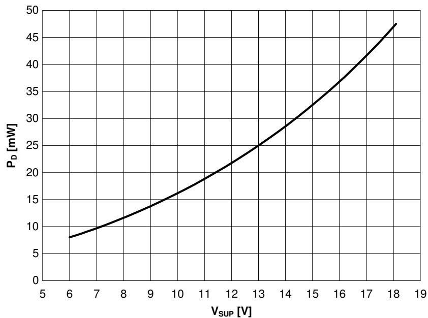
Figure 16 - Power dissipation LIN transceiver @ 20kbit
