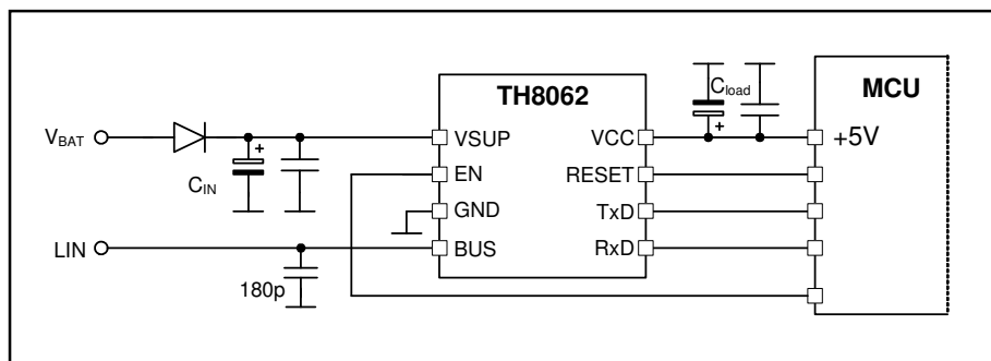
Figure 14 - EN controlled via MCU
