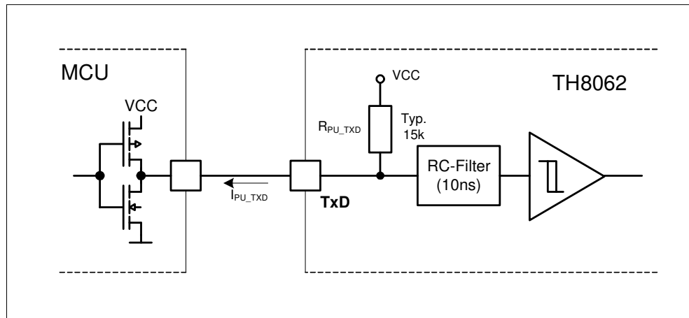
Figure 8 - TxD input circuitry
