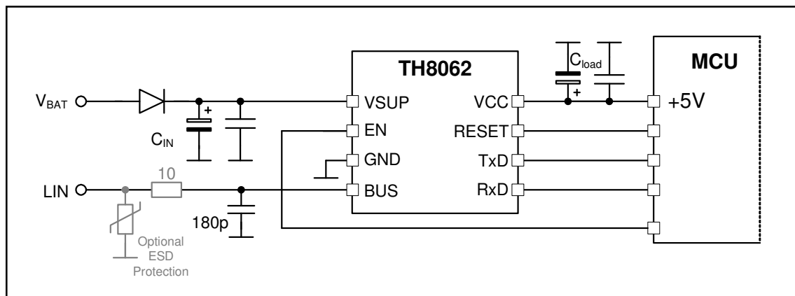
Figure 19 - Application circuit (slave node)
