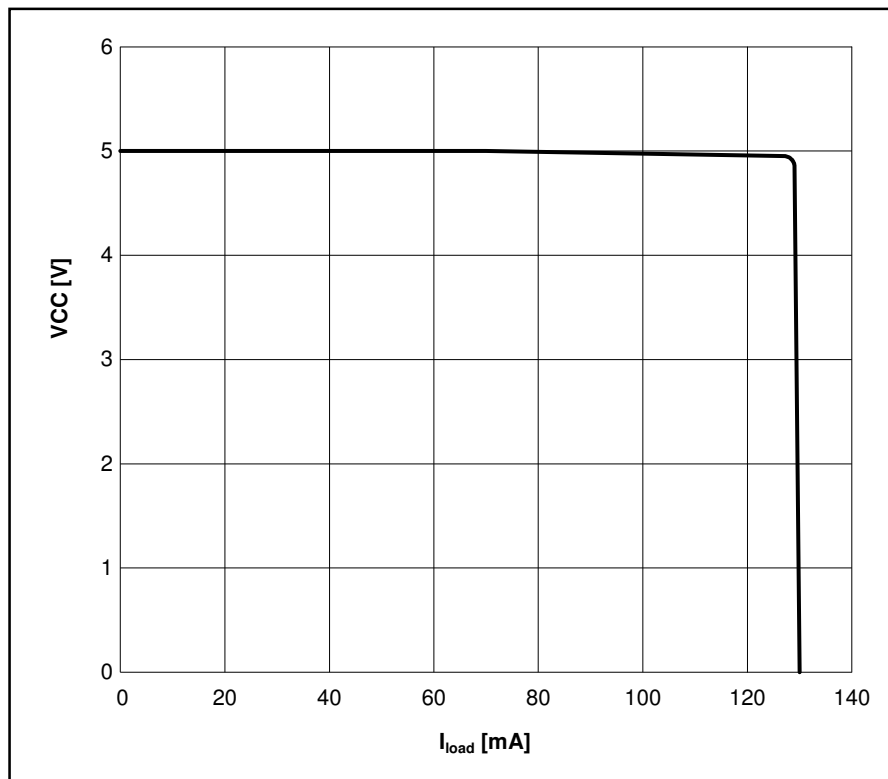
Figure 10 - Characteristic of current limitation V_{\text{CC}} = f(I_{\text{VCC}})
