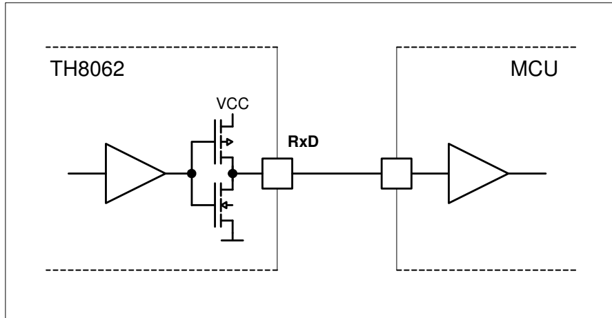
Figure 9 - RxD output circuitry
