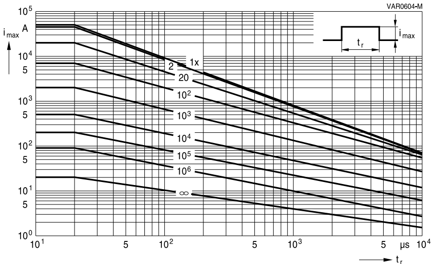
SIOV-LS41K230QP(K2) ... K460QP(K2)
