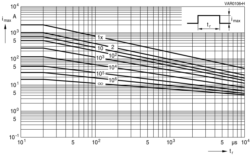
SIOV-S20K11 ... K40
