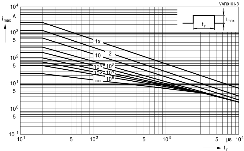
SIOV-S10K50 ... K320
