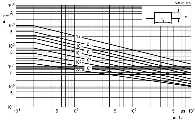
SIOV-S14K11 ... K40
