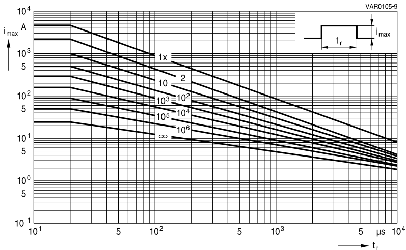
SIOV-S14K385 ... K1000
