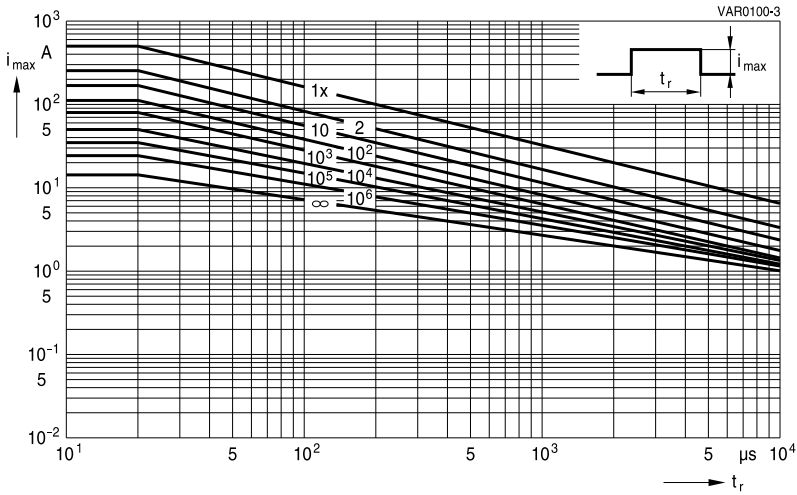
SIOV-S10K11 ... K40
