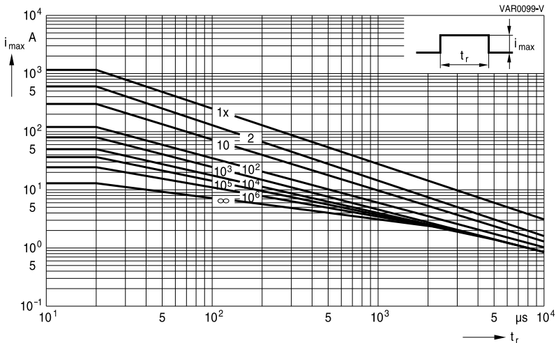
SIOV-S07K50 ... K460
