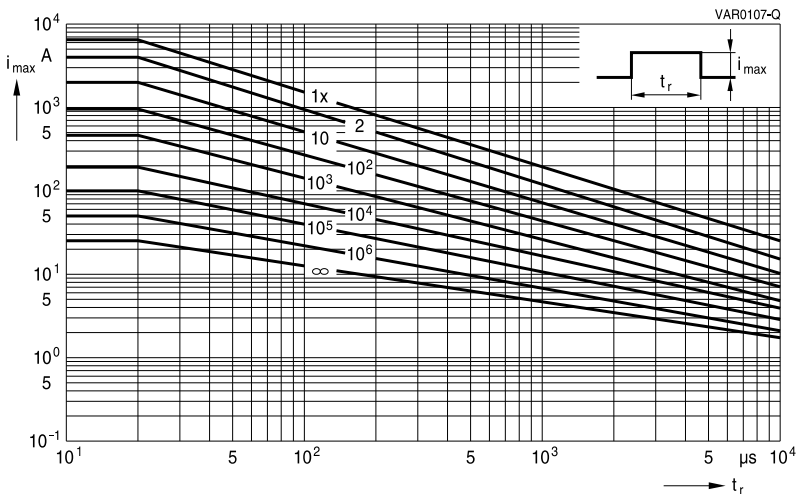
SIOV-S20K50 ... K115
