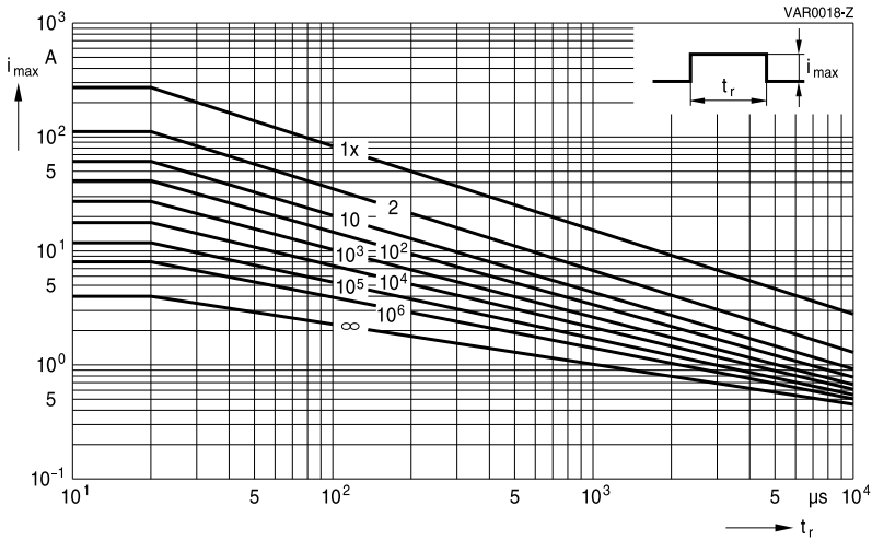
SIOV-S07K11 ... K40
