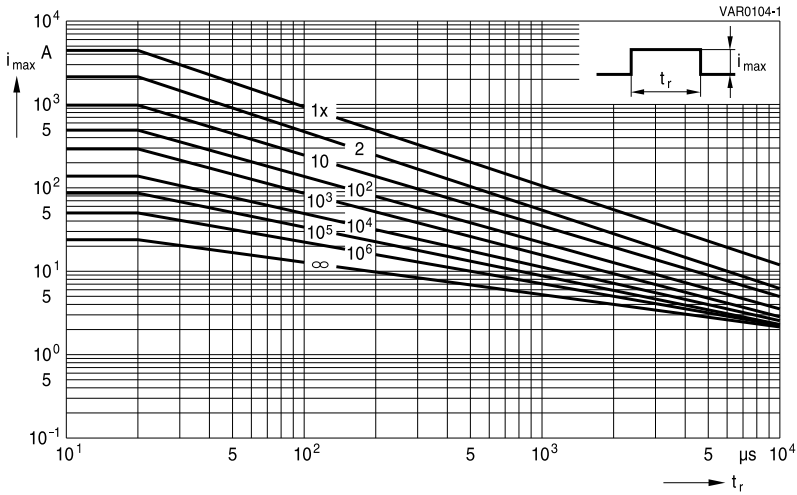
SIOV-S14K50 ... K320
