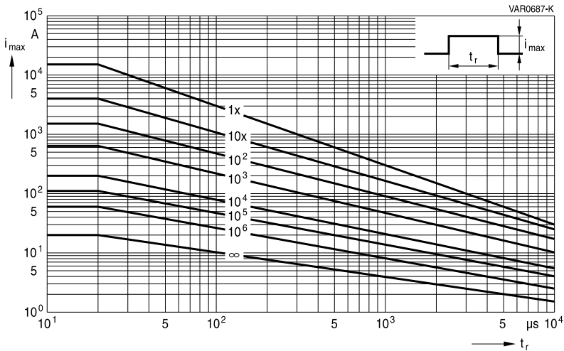
SIOV-Q20K350 ... K460
