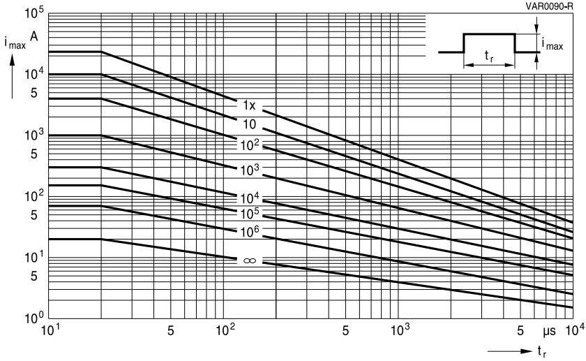
SIOV-B32K550 ... K750
