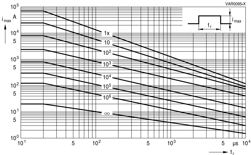
SIOV-B60K230 ... K460
