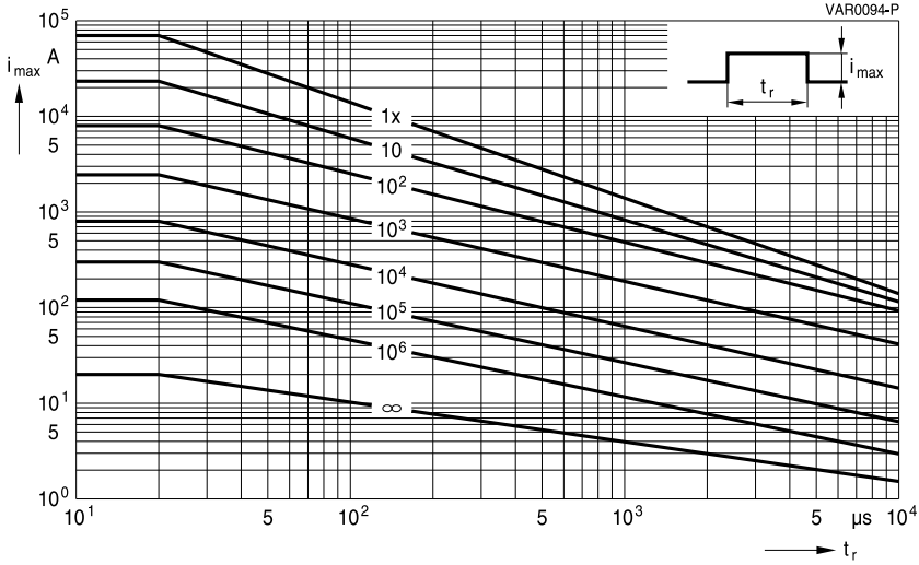
SIOV-B60K130 ... K150
