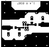
Optimised PCB layout for SAW filters in DCC6F package, pinning 1,4 (top side, scale 1:1)
