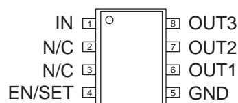
AAT4291A SC70JW-8 (Top View)
