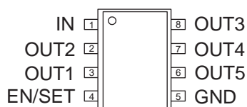
AAT4290A SC70JW-8 (Top View)
