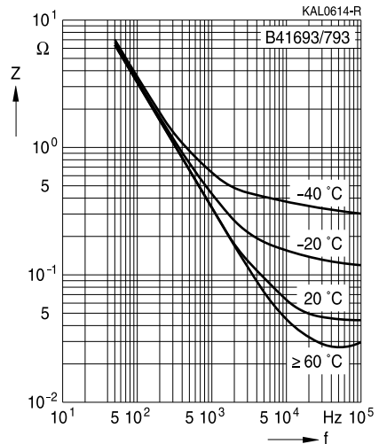
Impedance Z versus frequency f Typical behavior for 470 \mu F/63V
