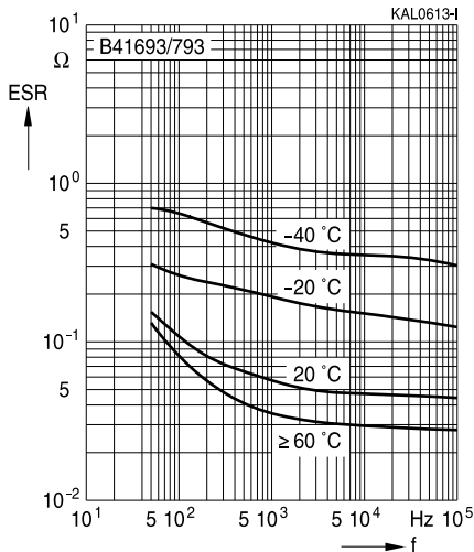
Equivalent series resistance ESR versus frequency f Typical behavior for 470 \mu F/63V
