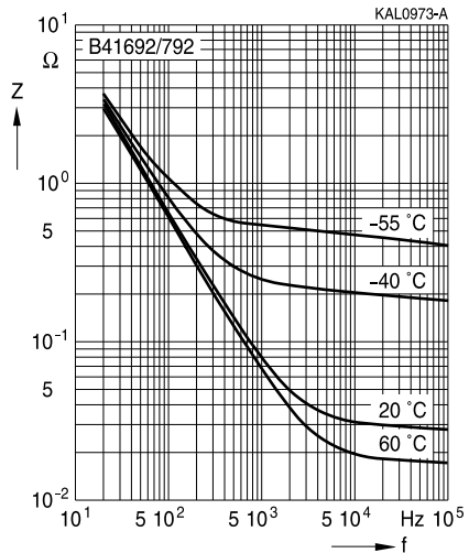
Impedance Z versus frequency f Typical behavior for 2200 \mu\text{F}/25\text{ V}
