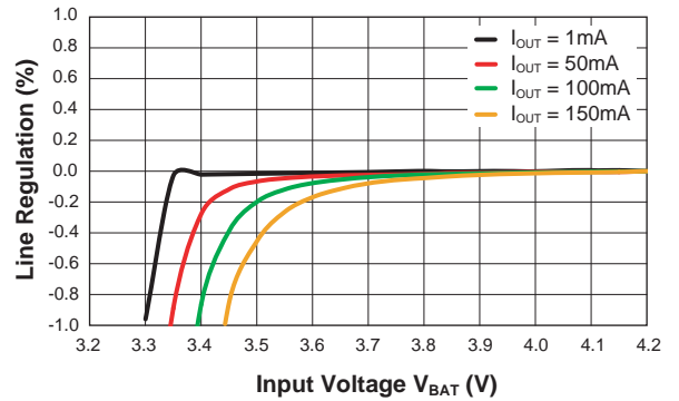
LDO5 Line Regulation vs. Battery Input Voltage ( V_{OUT} = 3.3V )
