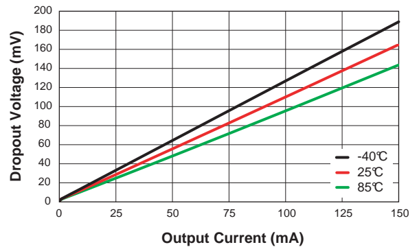
LDO2 Dropout Voltage vs. Output Current ( V_{OUT} = 1.2V )
