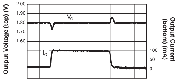
Time (100µs/div)
