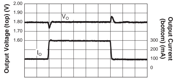
Time (100µs/div)
