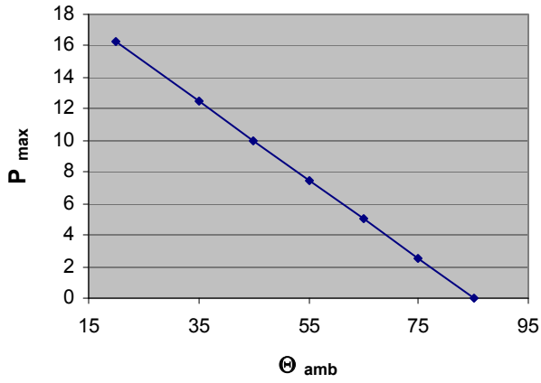
Max. allowable power loss at specific ambient Temp. B32344E4152A010
