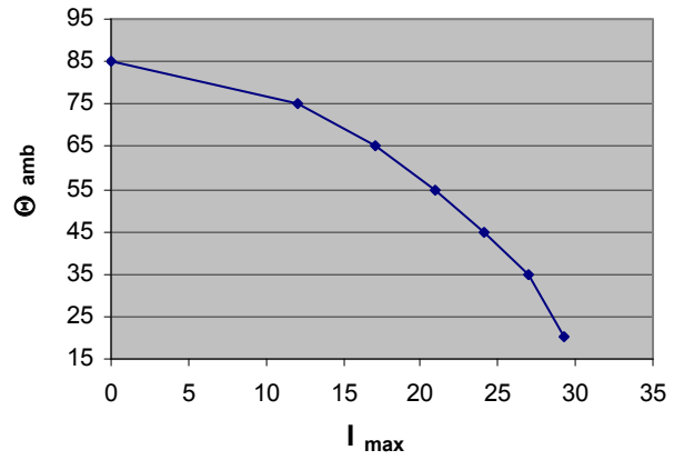
Max. allowable ambient Temp. at specific current (rms) B32344E4152A010
