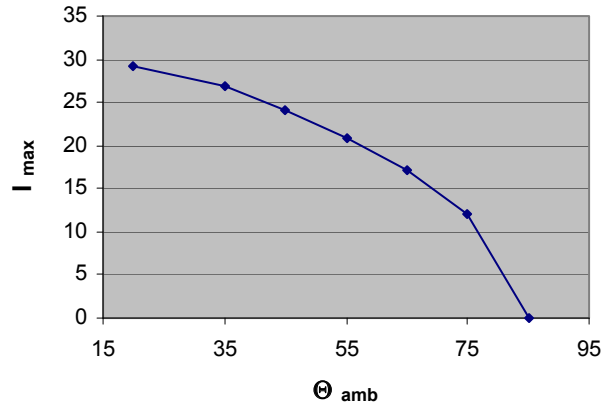
Max. allowable current (rms) at specific ambient Temp. B32344E4152A010
