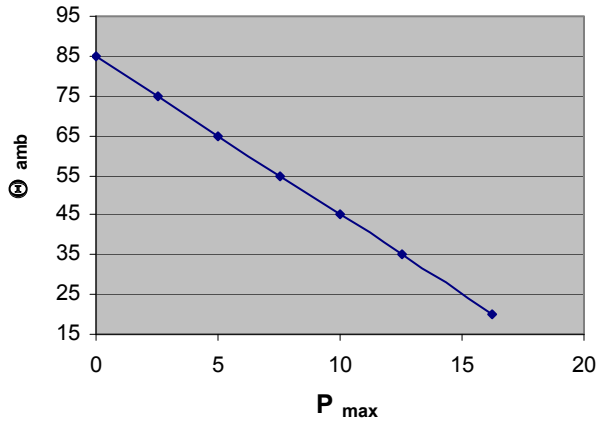
Max. allowable ambient Temp. at specific power loss B32344E4152A010
