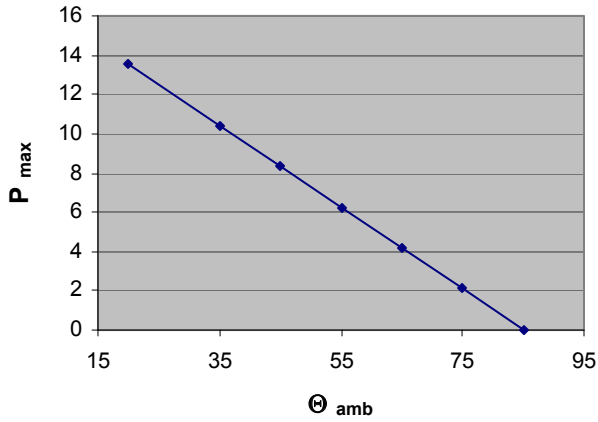
Max. allowable power loss at specific ambient Temp. B32344E4151A080
