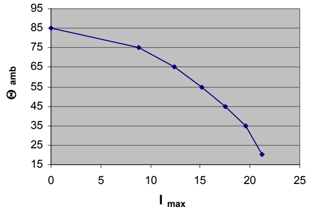
Max. allowable ambient Temp. at specific current (rms) B32344E4151A080
