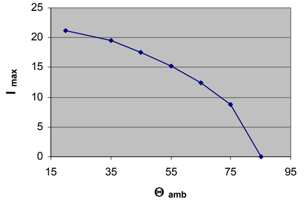
Max. allowable current (rms) at specific ambient Temp. B32344E4151A080
