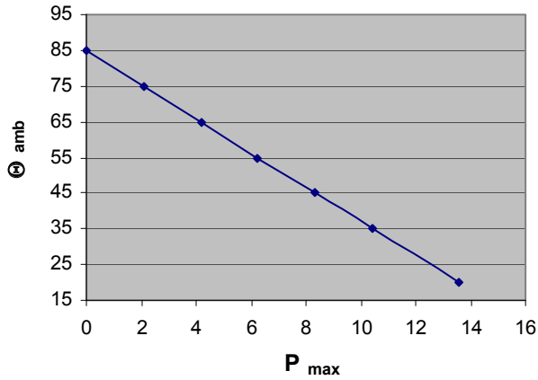
Max. allowable ambient Temp. at specific power loss B32344E4151A080
