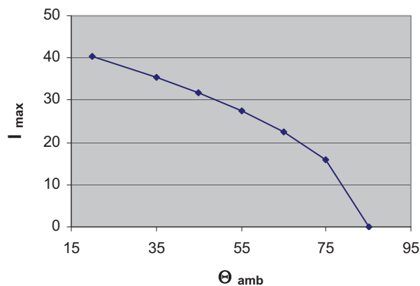
Max. allowable current (rms) at specific ambient Temp. B25673S5252A020
