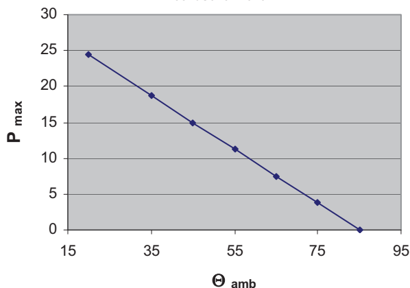
Max. allowable power loss at specific ambient Temp. B25673S5252A020
