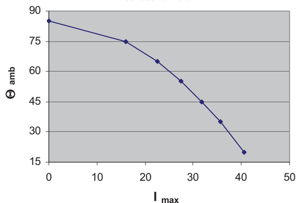
Max. allowable ambient Temp. at specific current (rms) B25673S5252A020
