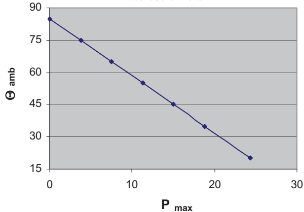
Max. allowable ambient Temp. at specific power loss B25673S5252A020
