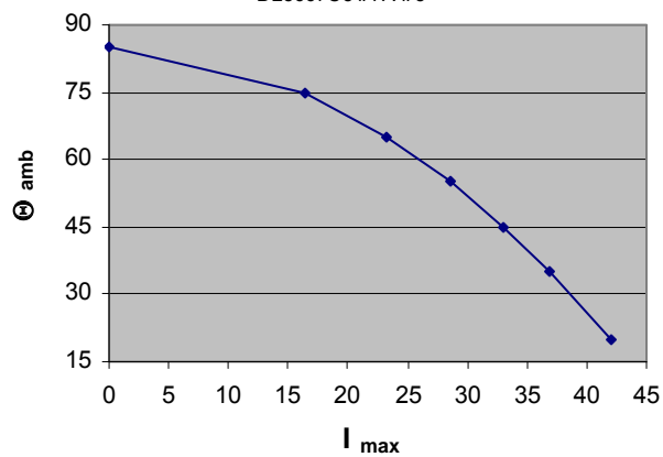
Max. allowable ambient Temp. at specific current (rms) B25667C5177A 175
