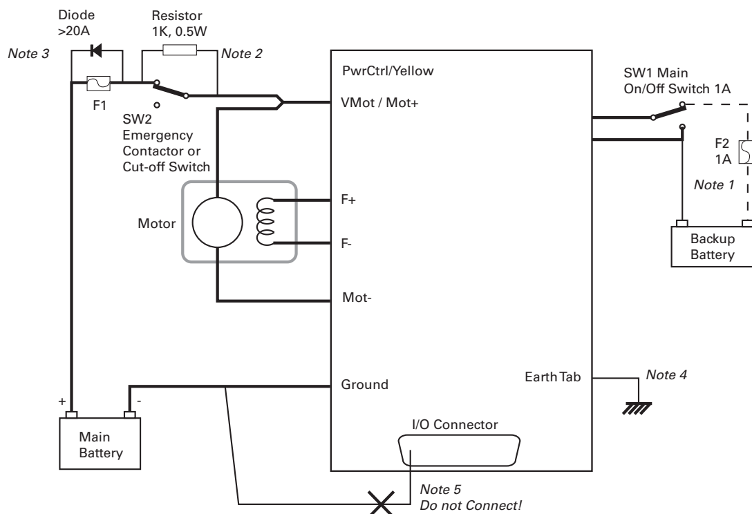
FIGURE 10. Powering the controller. Thick lines identify MANDATORY connections
