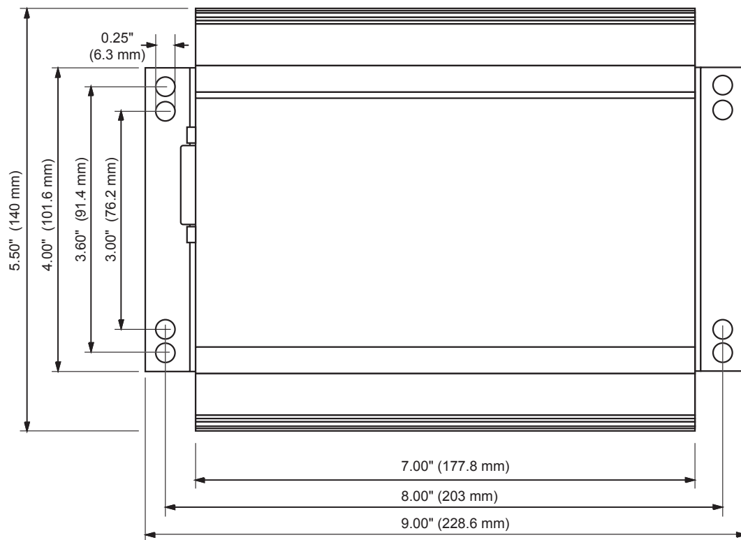
FIGURE 18. VSX1850 top view and dimensions
