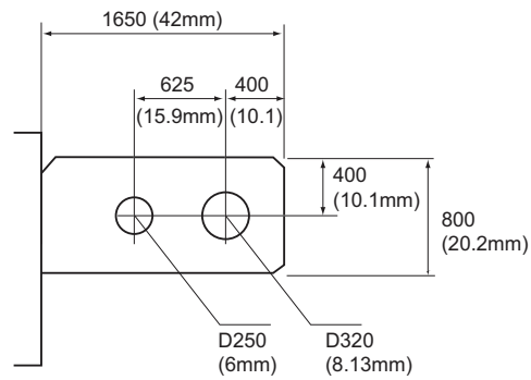
FIGURE 17. High Current copper bar connectors
