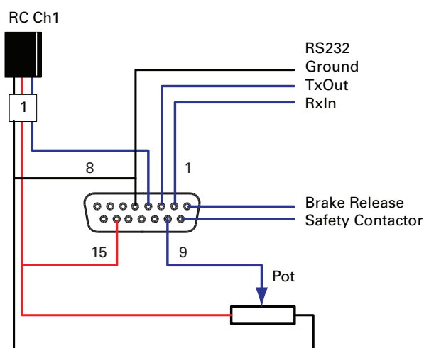
FIGURE 13. Factory default pins assignment
