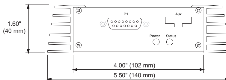
FIGURE 16. VSX1850 front view and dimensions
