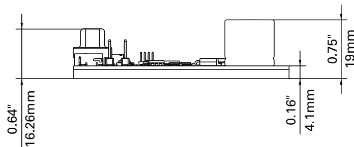
FIGURE 16. SDC2130/SDC2150 front view and dimensions
