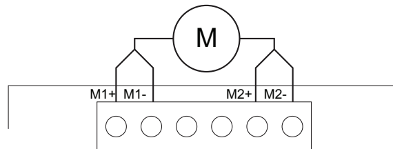
FIGURE 11. SDC2130S and SDC2150S wiring diagram
