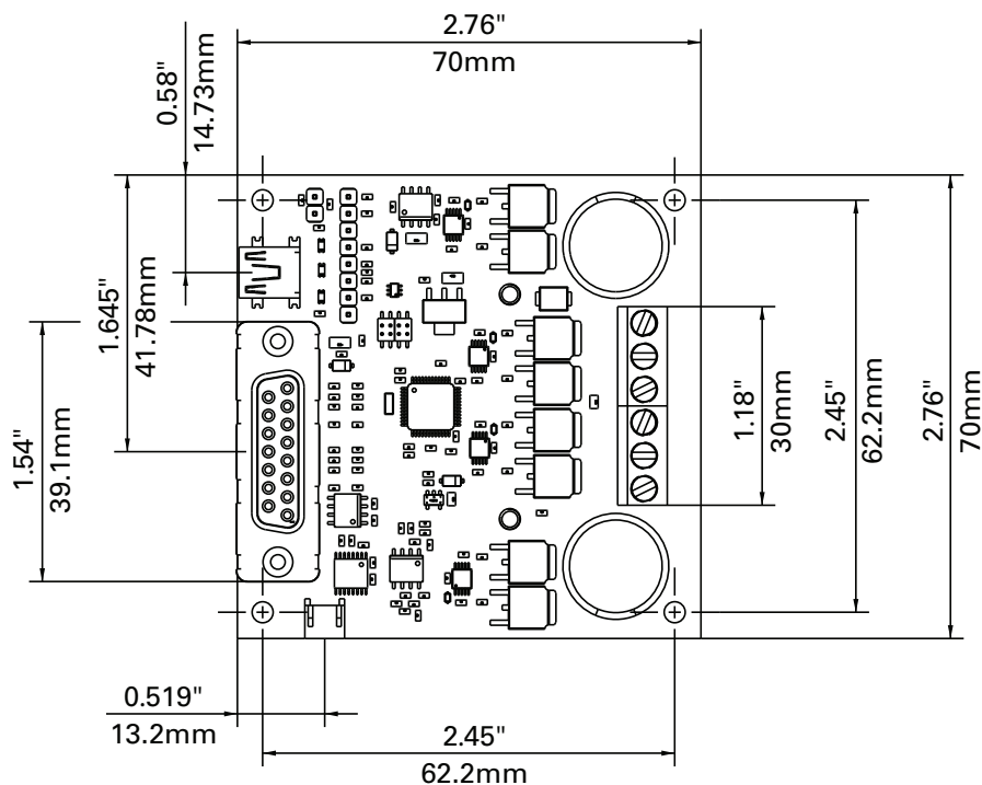
FIGURE 17. SDC2130/SDC2150 top view and dimensions
