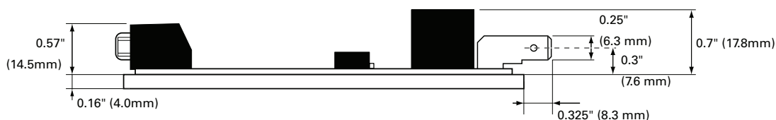
FIGURE 15. LDC1430/LDC1450 front view and dimensions
