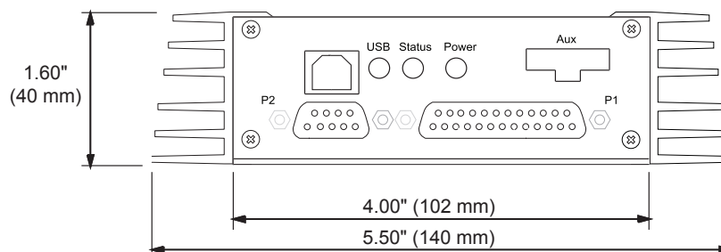
FIGURE 17. HDC2450 front view and dimensions
