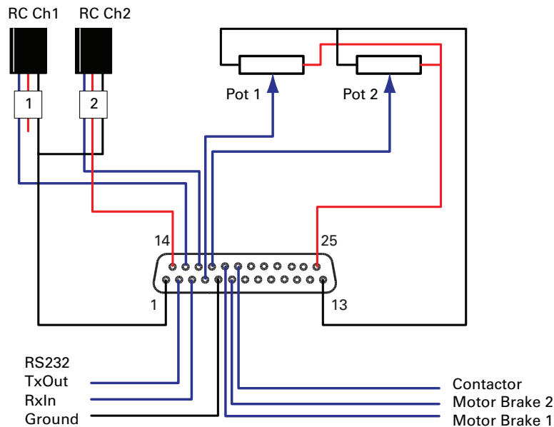
FIGURE 14. Factory default pins assignment
