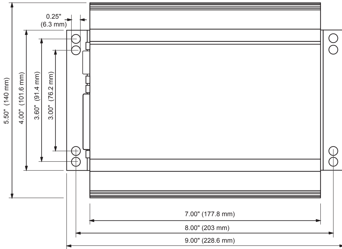
FIGURE 18. HDC2450 top view and dimensions
