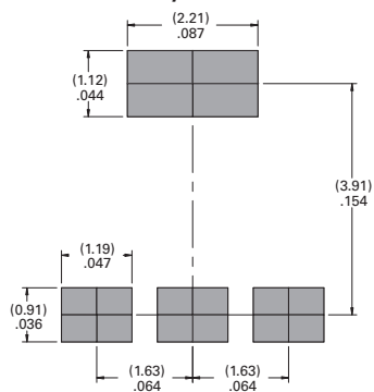
Pad Layout for SOT-89
