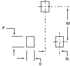
SP0502BAHT - SOT23-3
