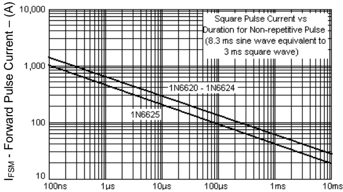
Pulse Duration FIGURE 7 Forward Pulse Current vs. Pulse Duration
