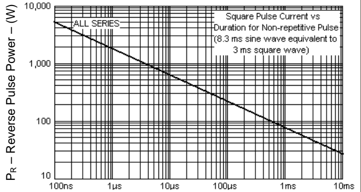
Pulse Duration FIGURE 8 Reverse Pulse Power vs. Pulse Duration
