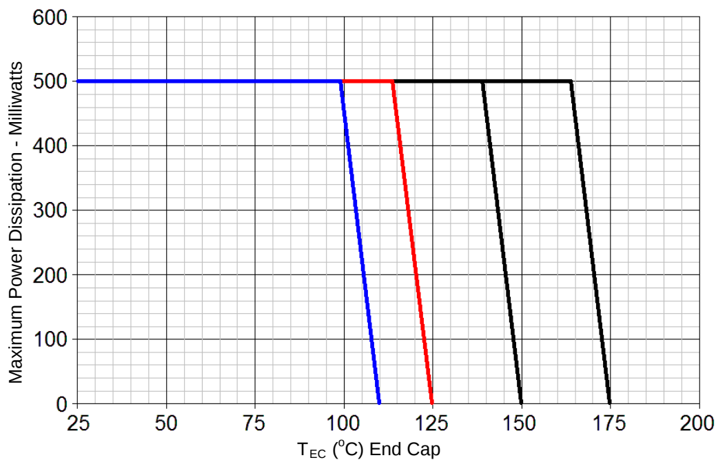
FIGURE 2 - (1N6321US – 1N6355US)
