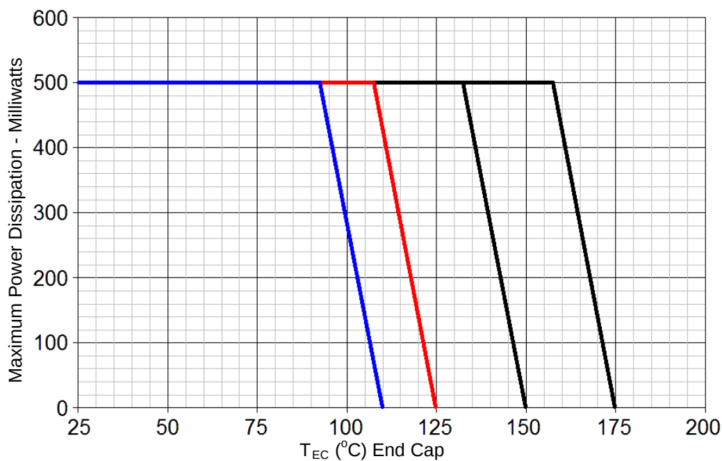
FIGURE 1 - (1N6309US – 1N6320US)
