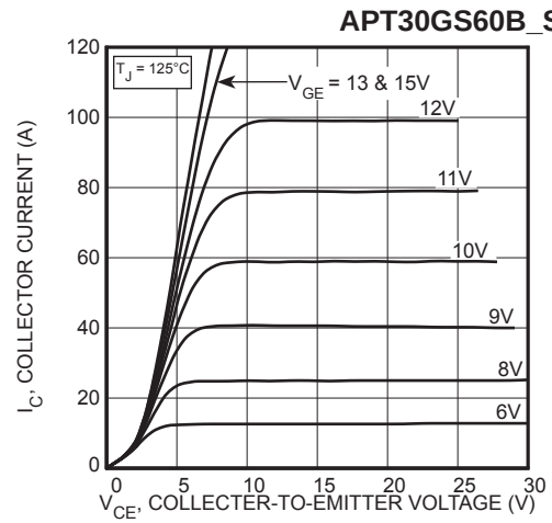
FIGURE 2, Output Characteristics
