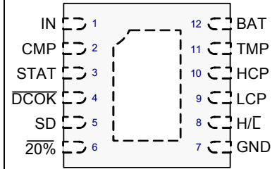
LD Package (Top View)
