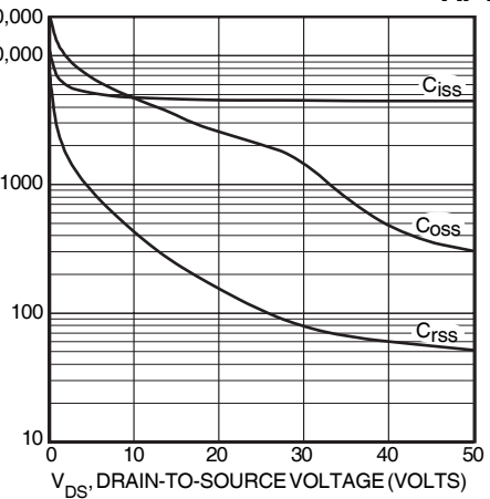
FIGURE 11, CAPACITANCE vs DRAIN-TO-SOURCE VOLTAGE
