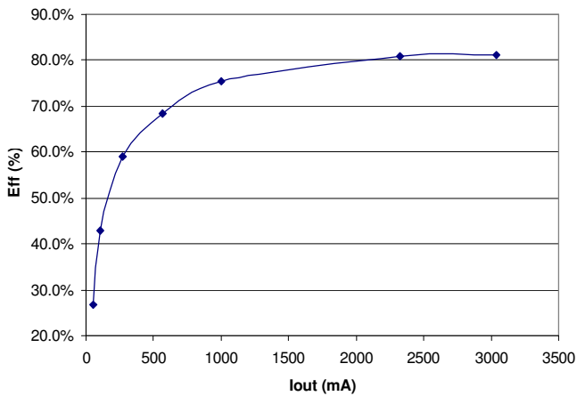
Figure 11 - Efficiency (VIN=30V,VOUT=5V)
