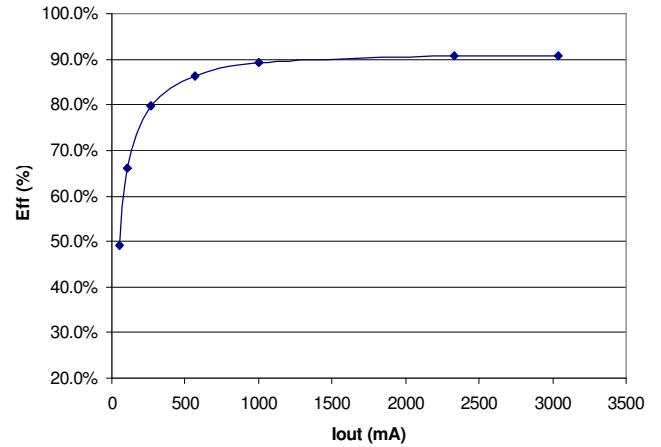
Figure 10 - Efficiency (VIN=12V,VOUT=5V)
