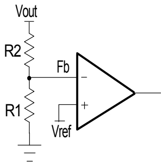
Figure 11 - Voltage Divider
