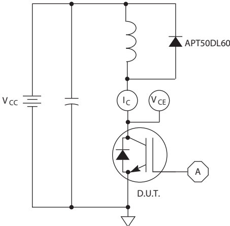
Figure 21, Inductive Switching Test Circuit
