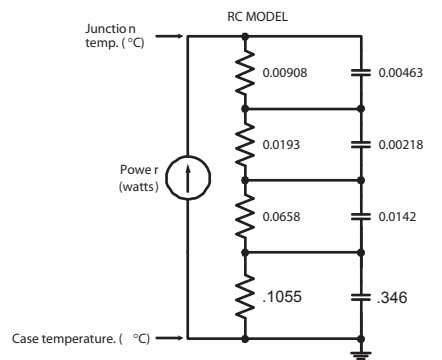
FIGURE 19b, TRANSIENT THERMAL IMPEDANCE MODEL
