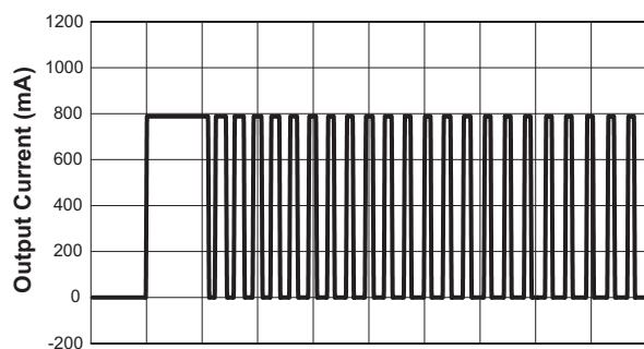
Over-Current Protection
