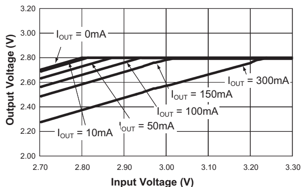
Dropout Characteristics
